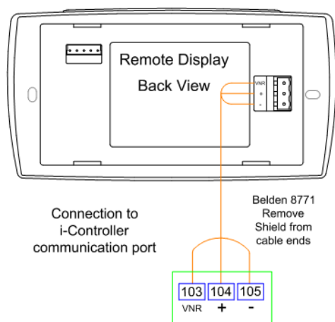
Figure 9. Visograph Connections
