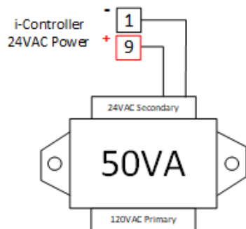
Figure 2. 24VAC Transformer
