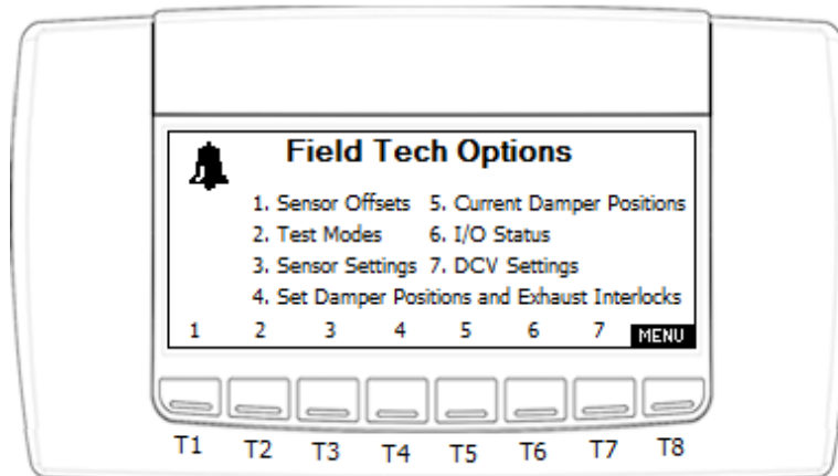
Figure 22. Visograph Field Tech Options screen
