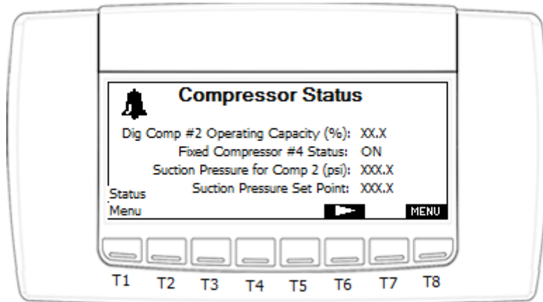
Figure 10. Visograph Compressor Status screen 1
