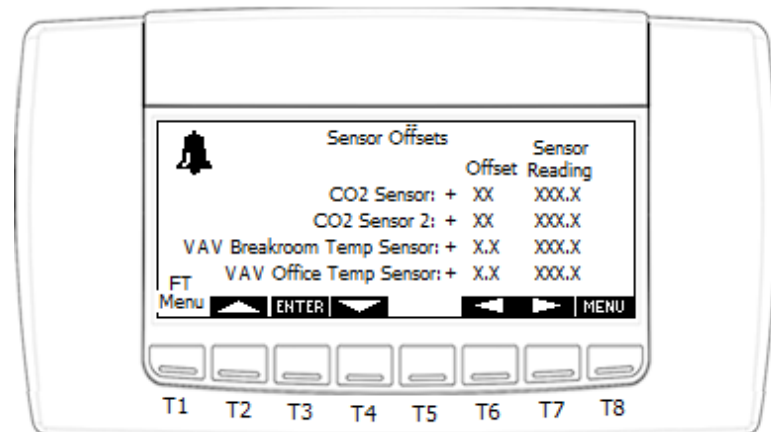
Figure 26. Visograph Sensor Offsets screen 4
