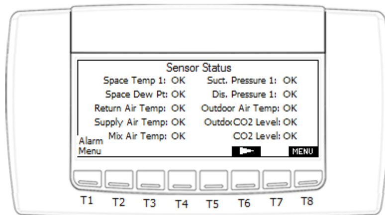
Figure 17. Visograph Sensor Status screen 1
