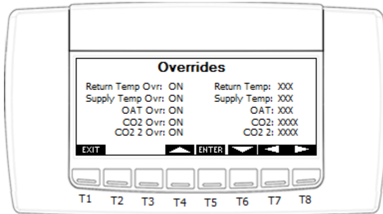
Figure 49. Visograph Overrides screen 3
