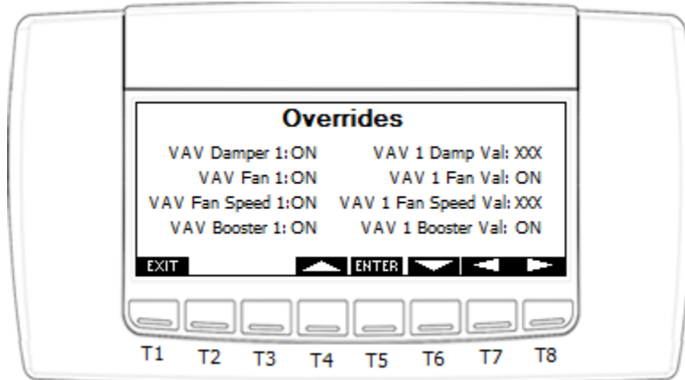
Figure 56. Visograph VAV Overrides screen 2
