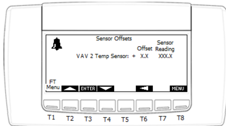
Figure 27. Visograph Sensor Offsets screen 5
