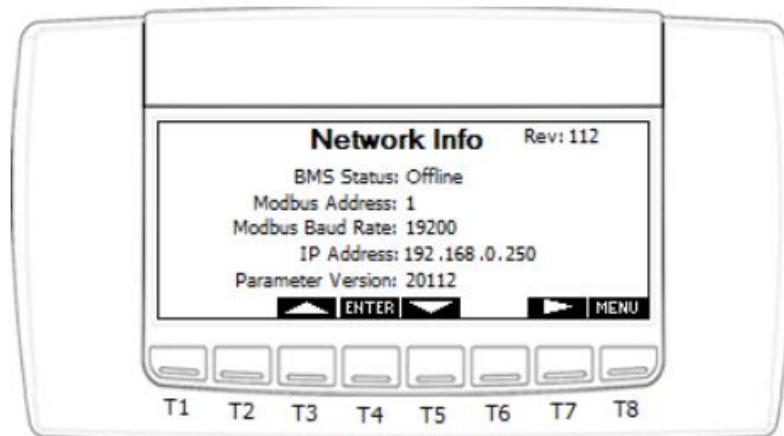
Figure 19. Visograph Network Information screen 1
