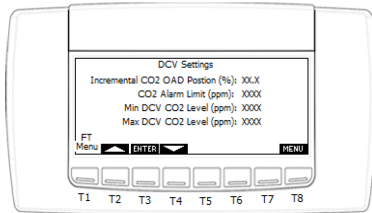
Figure 44. Visograph DCV Settings screen
