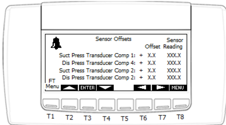
Figure 25. Visograph Sensor Offsets screen 3
