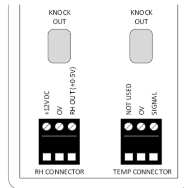
Figure 5.1. 203-5752 Space Temp/Humidity Terminal Connections
