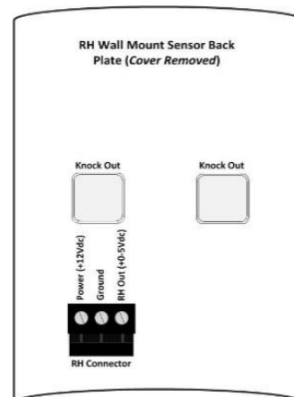
Figure 5.2. 203-5751 Humidity Terminal Connections
