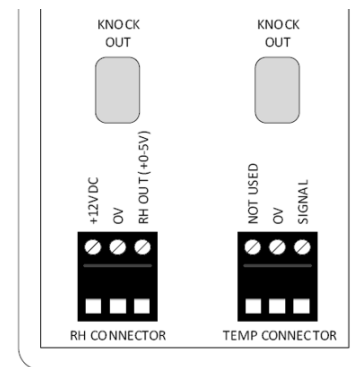
Figure 5.1. 203-5752 Space Temp/Humidity Terminal Connections
